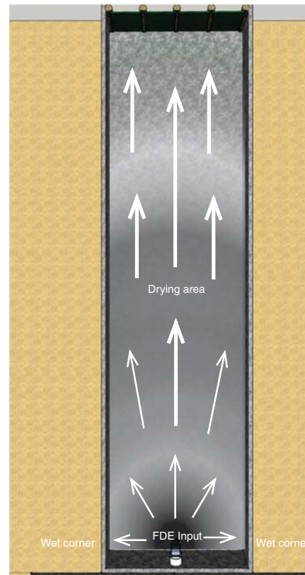
Type 1 with single point FDE input
